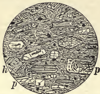
Fig. 35. — Hornblende-Andesite (trachytic type). Summit of Beinn Nevis, Scotland. \times 7 . h , Brown hornblende. p , Plagioclase, often much corroded by the glass around. Fluidal hemicrystalline groundmass.
